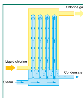
1b Steam bayonet
